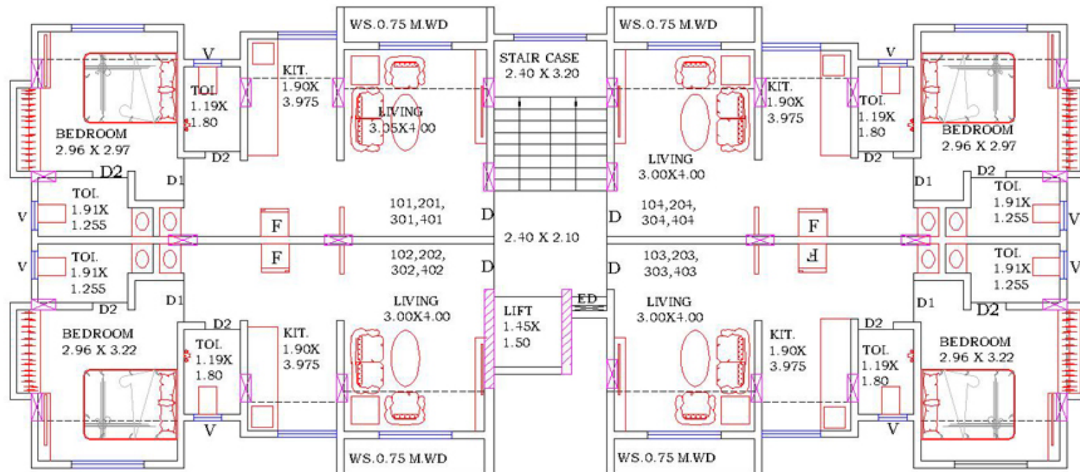
BLDG -A TYPICAL 1ST TO 4TH FLOOR PLAN
